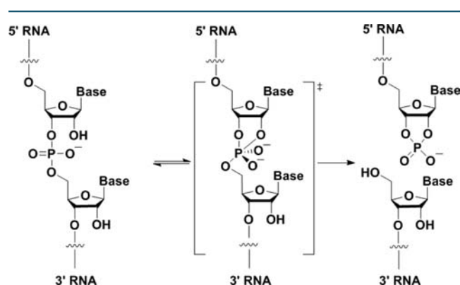
Figure 1. RNA Cleavage via phosphodiester transesterification.
